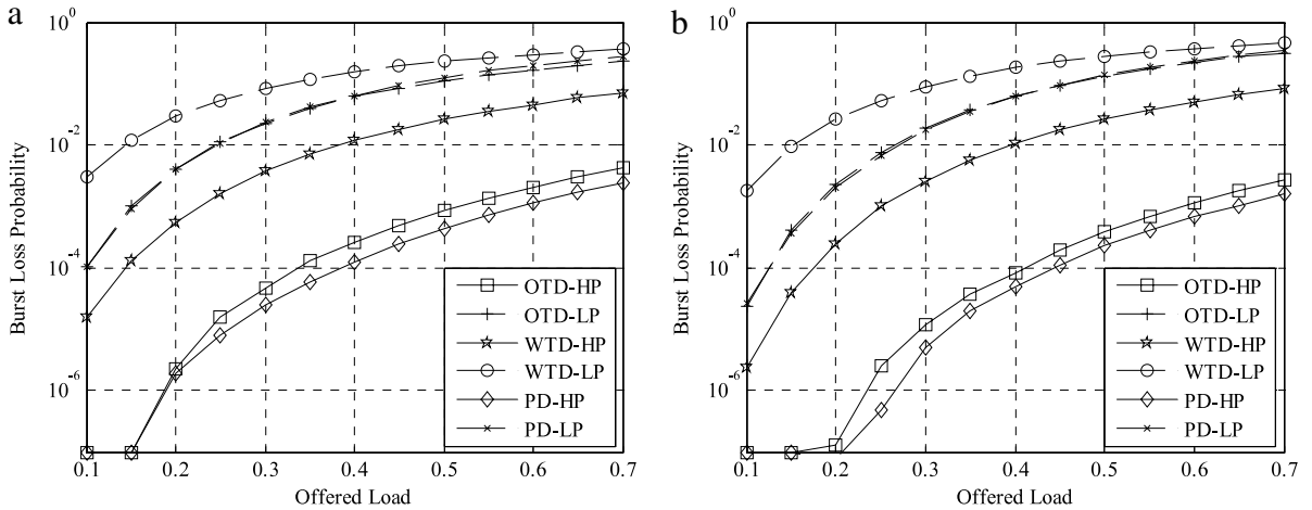
Fig. 6. Burst loss probability as a function of the offered load comparing OTD, WTD, and PD mechanisms when 30% of bursts are HP. (a) Poisson traffic model, (b) Gaussian traffic model.
