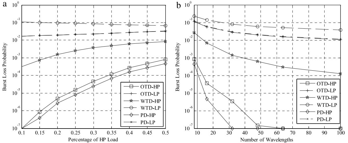
Fig. 7. Burst loss probability comparing OTD, WTD, and PD mechanisms as a function of: (a) percentage of HP load (Poisson model, offered load = 0.3, W = 8 ), (b) number of wavelengths, W (Poisson model, offered load = 0.5, 30% HP bursts).
