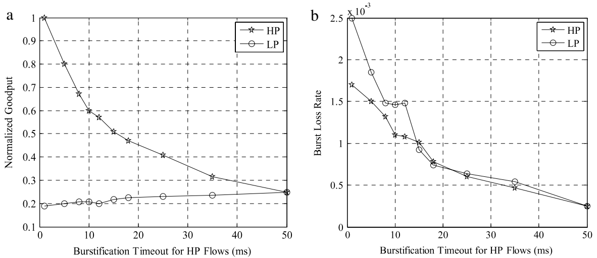
Fig. 9. Average normalized goodputs and burst loss rates as a function of HP burstification timeout for BLD mechanism.
