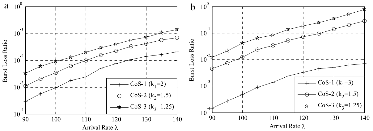
Fig. 10. Data loss ratio for three different classes of services with (a) k_i = 2, 1.5, and 1.25, (b) k_i = 3, 1.5 and 1.25, respectively, for i = 1, 2 and 3.
