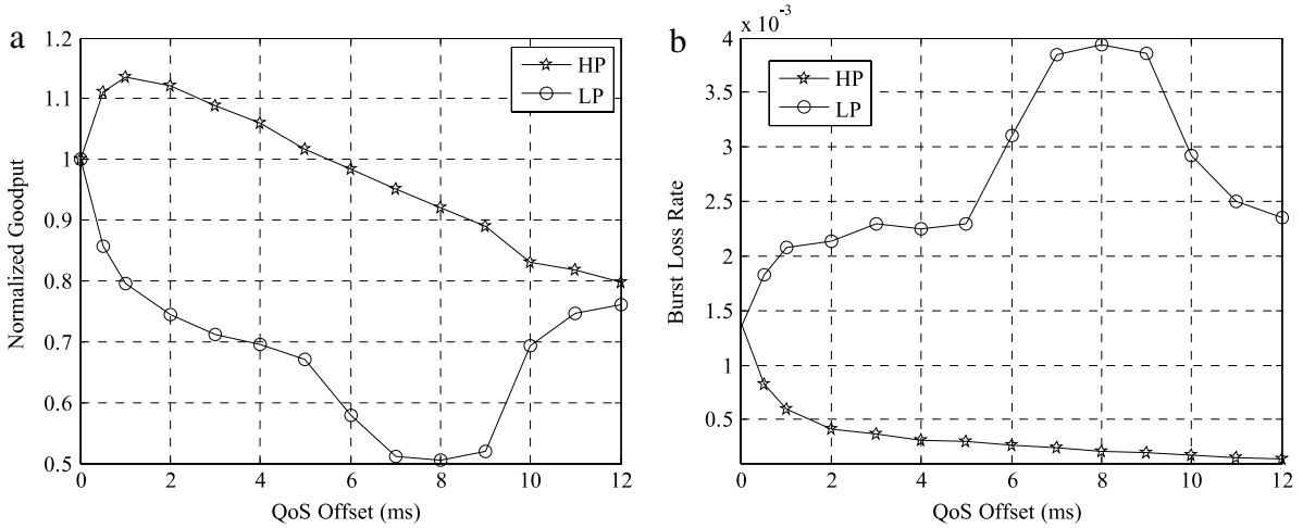
Fig. 8. Average normalized goodputs and burst loss rates as a function of QoS offset for OTD mechanism.
